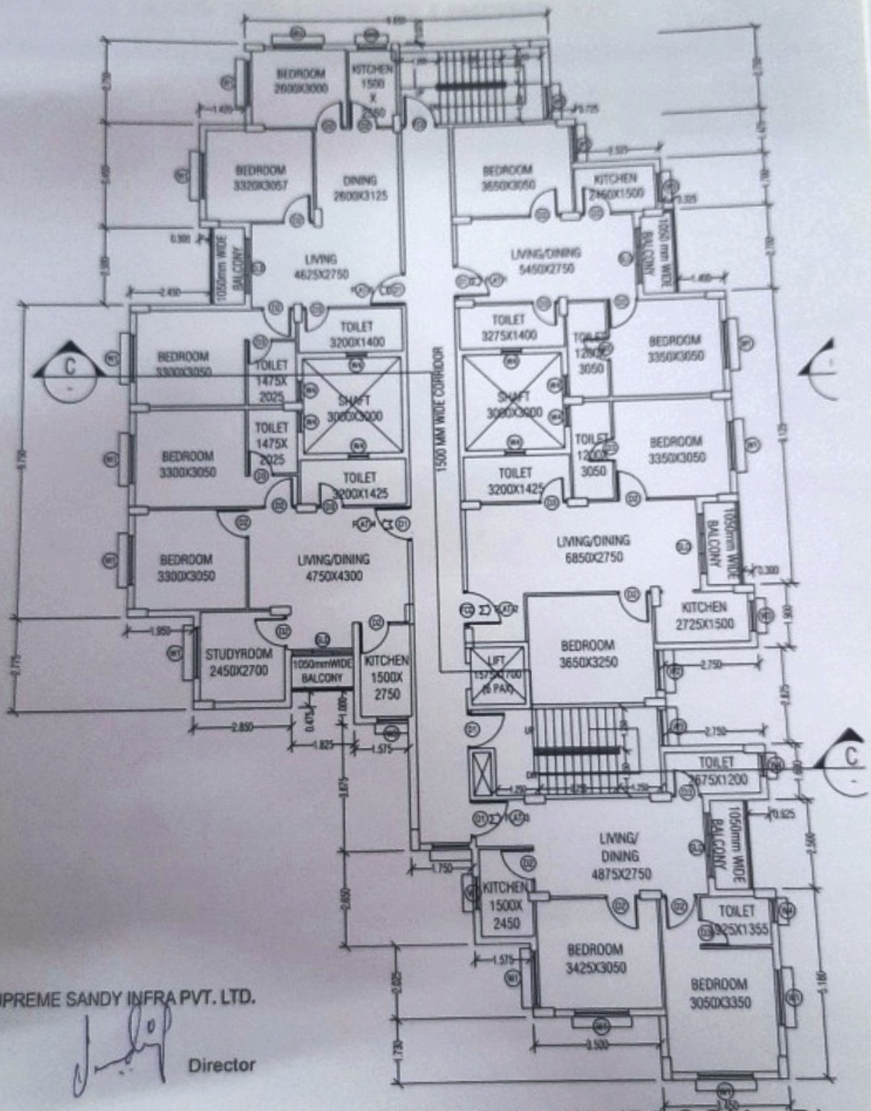
1 TYPICAL FLOOR PLAN (BLOCK - B) SCALE - 1:100
